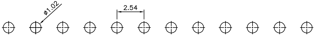
Recommended P.C.B. Layout
