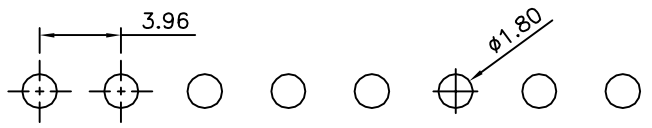
Recommended P.C.B. Layout(Component Side)
