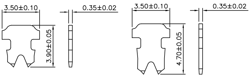
2 Prongs For Stranded Wire
