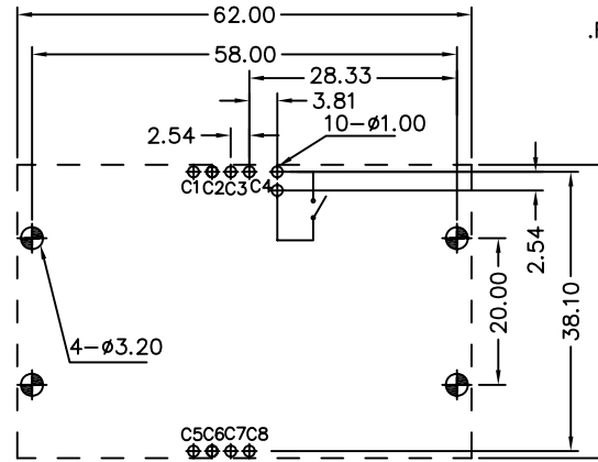
Reference P.C.B. Layout(Tolerance: ±0.10mm)
