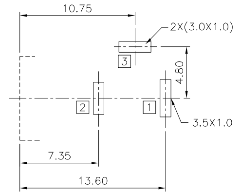
Recommended P.C.B. Layout(Bottom View) (PCB Board Tolerance±0.05)
