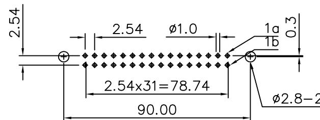
Layout Pattern
