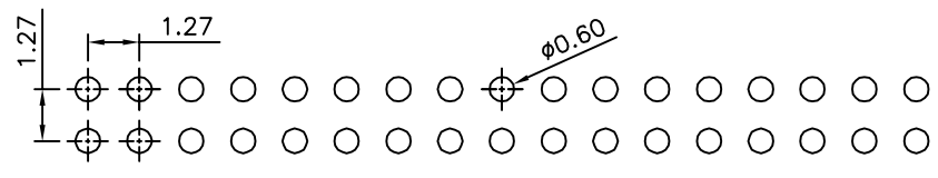
Recommended P.C.B. Layout(Top Side) (PCB Board Tolerance±0.05)
