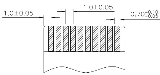
Proper Cable (T=0.3±0.02mm)
