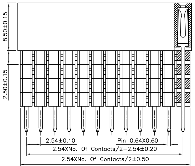
Section K-K
