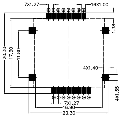
Reference P.C.B. Layout (Top View)
