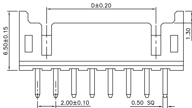
06~50 Pin Configuration
