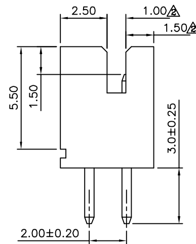
04 Pin Configuration
