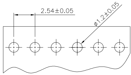
Recommended P.C.B. Layout PCB Board Thickness:1.6mm
