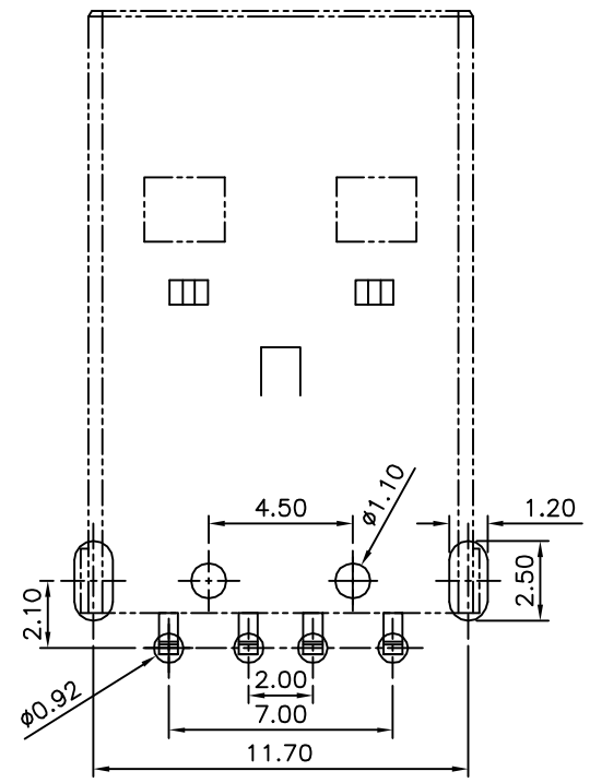
Recommended P.C.B. Layout Tolerances: ±0.10
