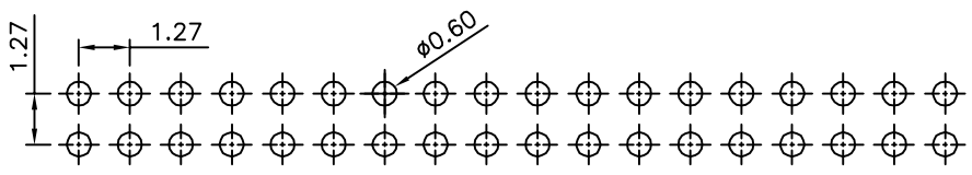
Recommended P.C.B. Layout(Top Side) (PCB Board Tolerance±0.05)
