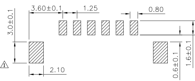
△ Recommended P.C.B. Layout(Top View) (PCB Board Tolerance±0.05)
