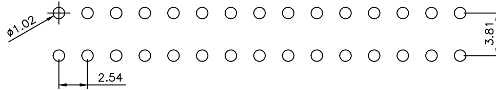
Recommended P.C.B Layout(Top Side) (PCB Board Tolerance \pm 0.05 )
