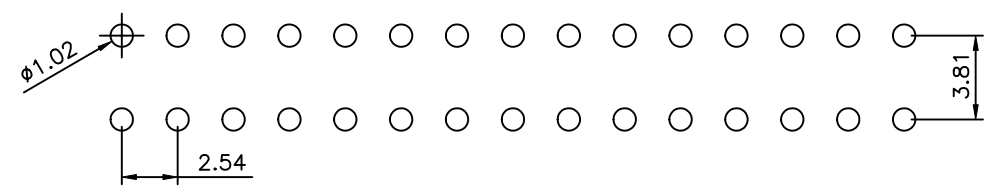
Recommended P.C.B Layout(Top Side) (PCB Board Tolerance±0.05)
