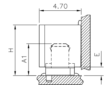
Mating Drawing(Ref)
