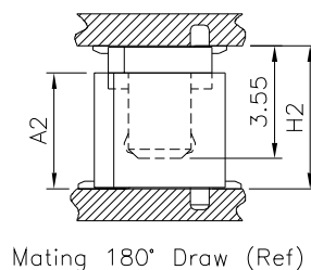
Mating 180° Dimension
