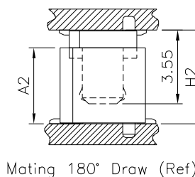
Mating 180° Dimension
