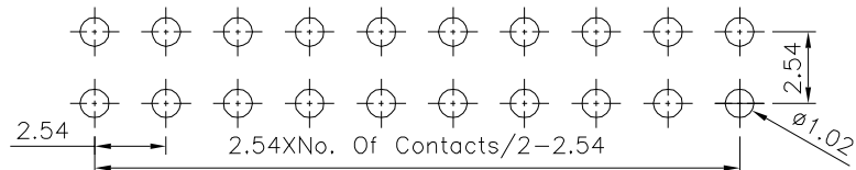
Recommended P.C.B. Layout(Top View)
