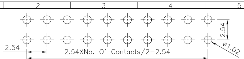
Recommended P.C.B. Layout(Top View) (PCB Board Tolerance±0.05)
