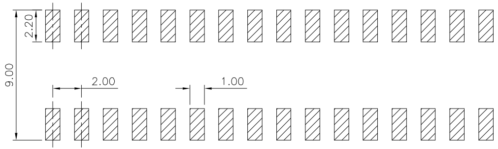
Recommended P.C.B. Layout (Top Side) \Delta (PCB Board Tolerance \pm 0.05 )
