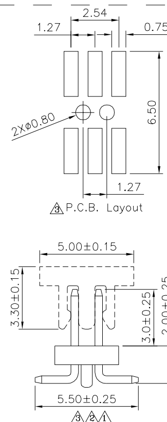
06 Pin
