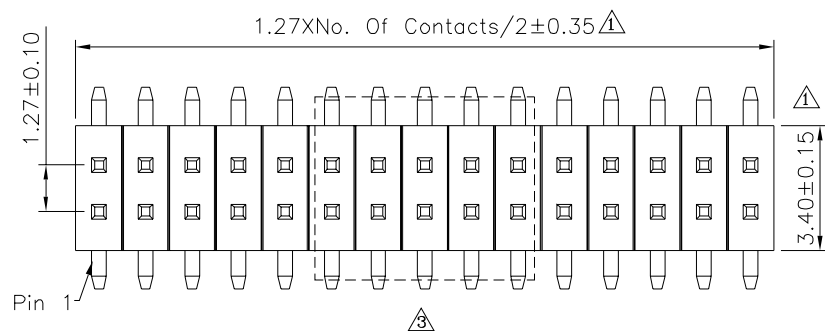
1.27X(No. Of Contacts/2-1)±0.20
