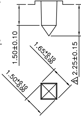
Detail K
