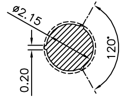
Detail J
