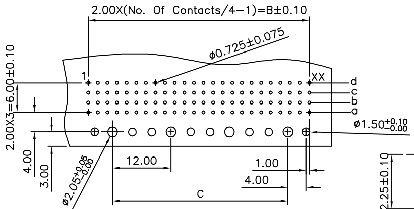
Recommended P.C.B. Layout (PCB Board Tolerance±0.05)
