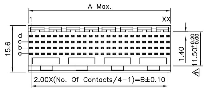
Recommended P.C.B. Layout (PCB Board Tolerance±0.05)
