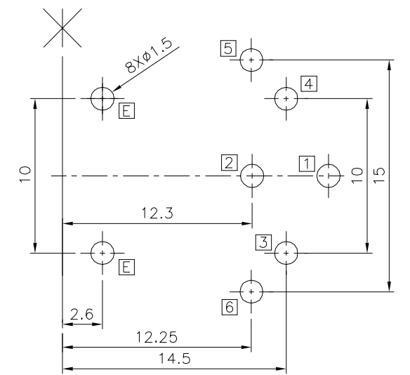
Recommended P.C.B. Layout(Copper-Side View)
