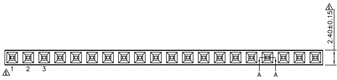
Recommended P.C.B. Layout(Top Side) (PCB Board Tolerance±0.05)
