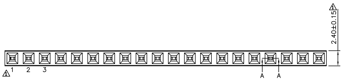
Recommended P.C.B. Layout(Top Side) (PCB Board Tolerance±0.05)
