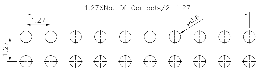
Recommended P.C.B. Layout(Top View) (PCB Board Tolerance±0.05)
