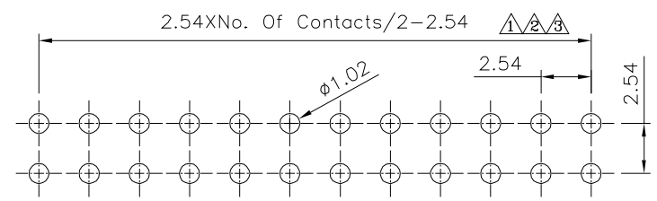
Recommended P.C.B. Layout Tolerance: ±0.05 (Top View)
