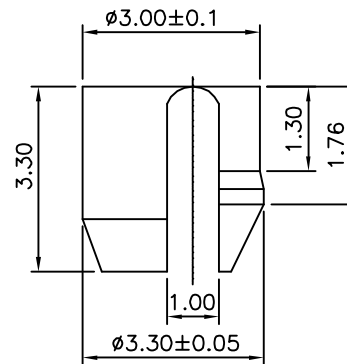
Detail X
