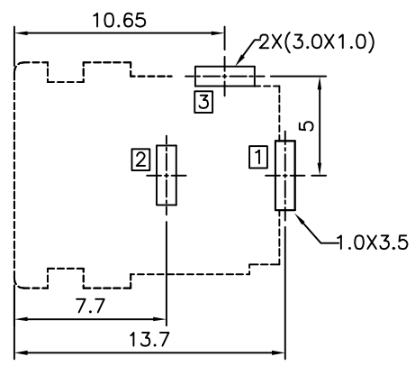
Recommended P.C.B. Layout(Bottom View) (PCB Board Tolerance±0.05)
