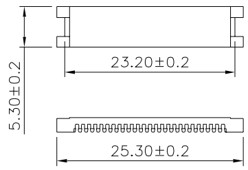
Termination Cover(2 PCS)
