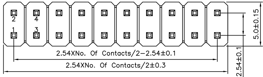
Recommended P.C.B. Layout(Top View) (PCB Board Tolerance±0.05)
