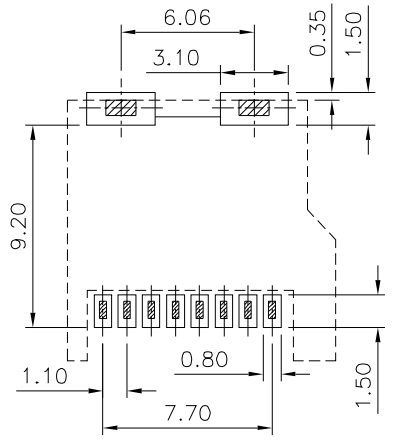
Recommended P.C.B. Layout(Component Side View) (PCB Board Tolerance±0.05)
