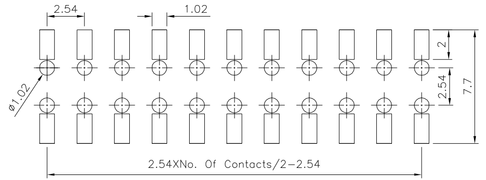
Recommended P.C.B. Layout(Top View) (PCB Board Tolerance±0.05)
