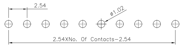
Recommended P.C.B. Layout(Top View) (PCB Board Tolerance±0.05)
