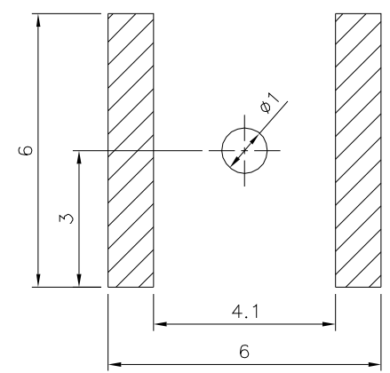
Recommended Mounting Holes
