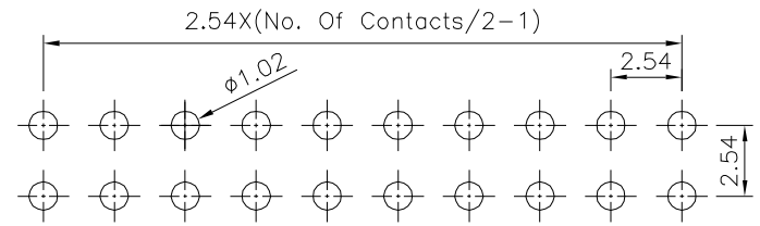
Recommended P.C.B. Layout PCB Tolerance:±0.05(Top View)
