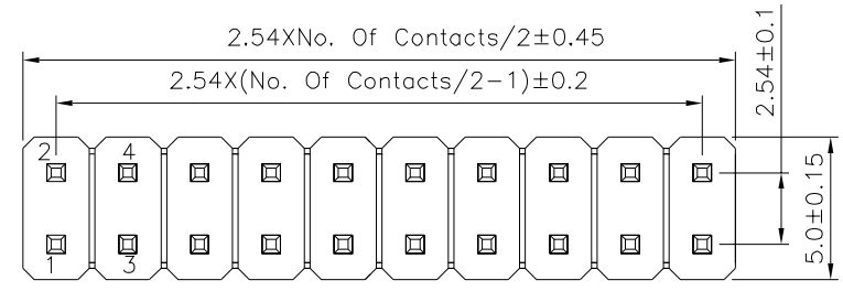
Recommended P.C.B. Layout PCB Tolerance:±0.05(Top View)
