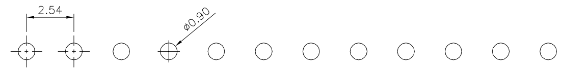
Recommended P.C.B. Layout △ Tolerance ±0.05
