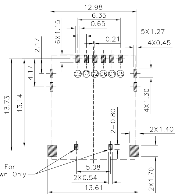
Recommended P.C.B. Layout (PCB Board Tolerance:±0.05)
