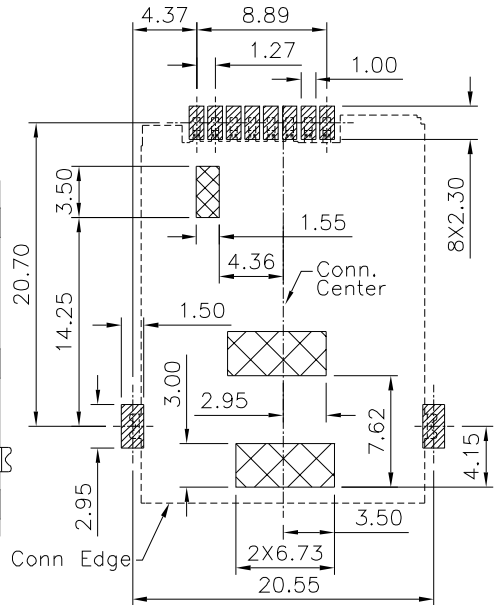
Recommended P.C.B. Layout (PCB Board Tolerance±0.05)
