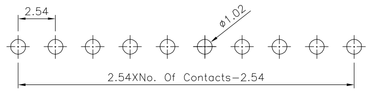
Recommended P.C.B. Board Layout PCB Tolerance: \pm 0.05 (Top View)
