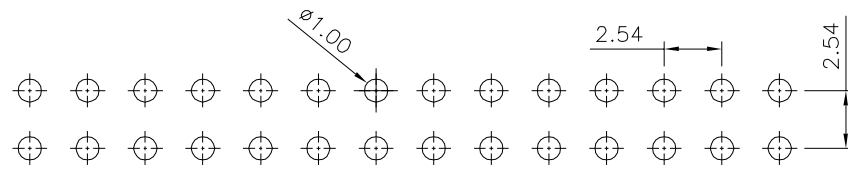
Recommended P.C.B. Layout ⚠ Tolerance \pm 0.05
