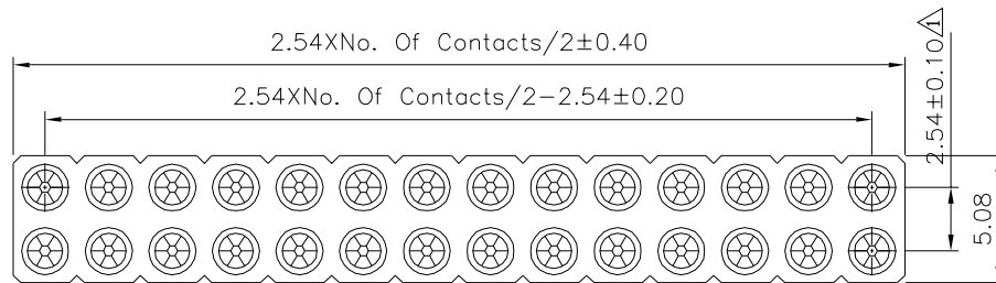
Recommended P.C.B. Layout ⚠ Tolerance \pm 0.05
