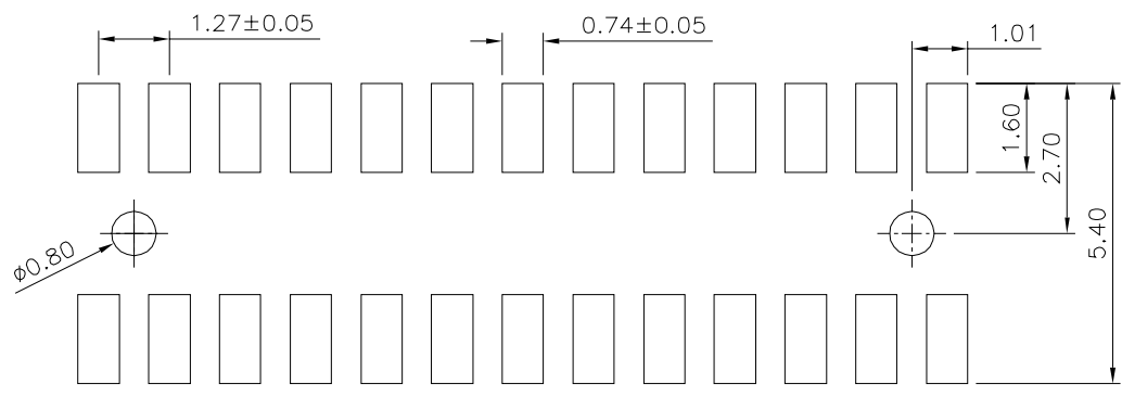
Recommended P.C.B. Layout (PCB Board Tolerance±0.05)
