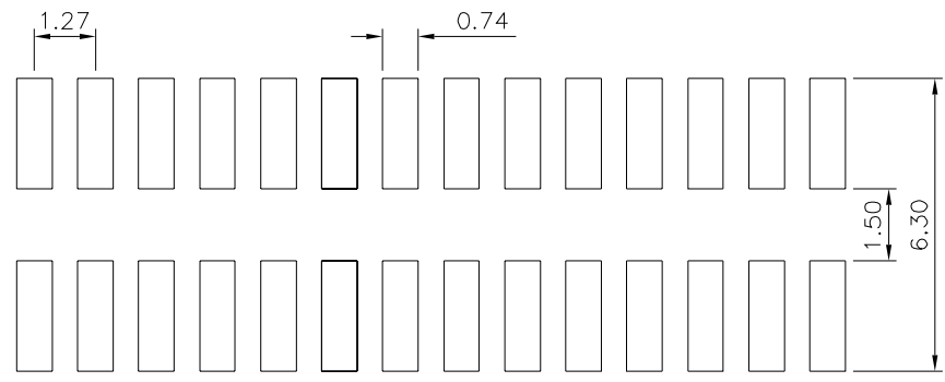
Recommended P.C.B. Layout PCB Board Tolerance±0.05
