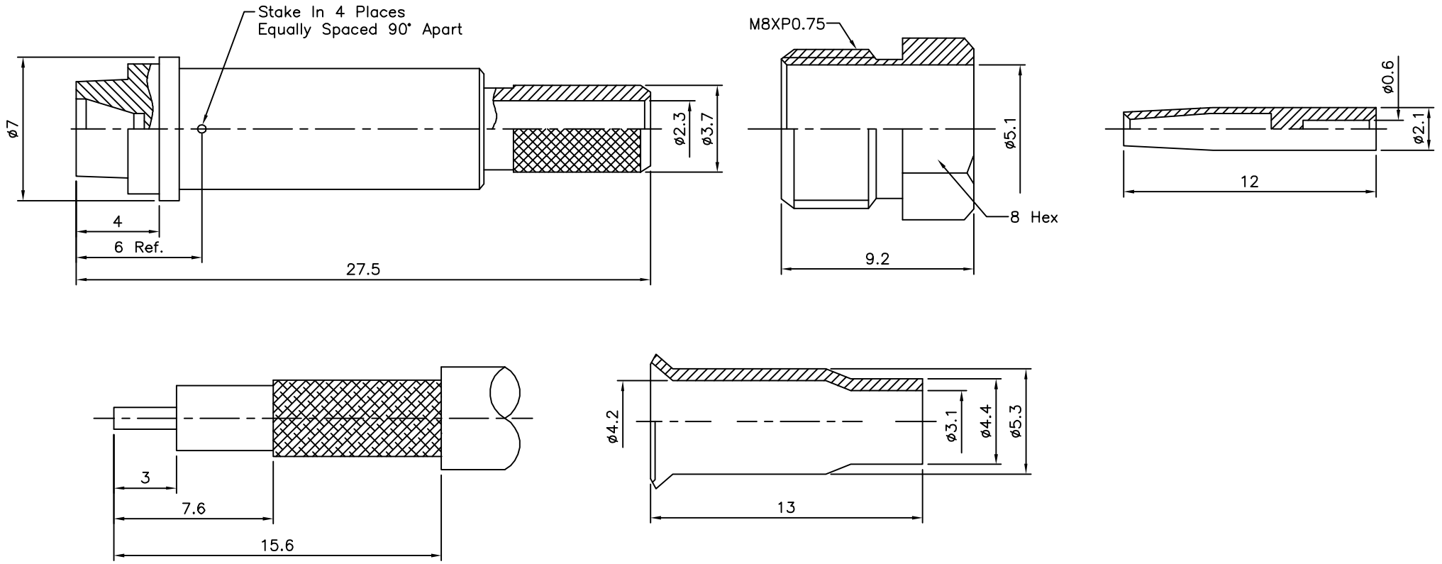
Recommended Cable Stripping Dimension
