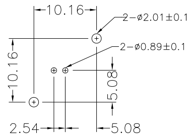
Recommended PC Board layout Without mounting posts
