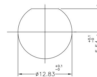
Recommended mounting hole maximun panel thickness:5.5mm
